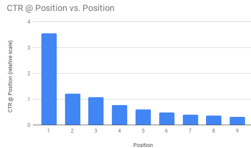
Figure 6: CTR for position 1 to 9.
