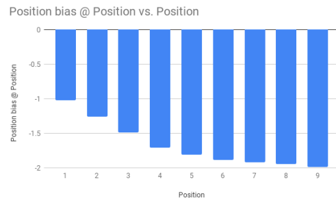
Figure 7: Learned position bias per position.
